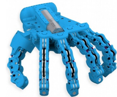
The SoftHand developed by the partners University Pisa and IIT.
