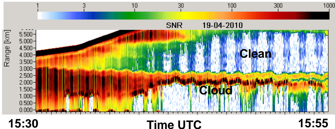
Figure 7: Quicklook from 2- \mu m lidar measurements from Falcon flight on April 19, 2010 showing Signal-to-Noise Ratio during 25 minutes from Leipzig to Hamburg from 15:30-15:55 UTC (17:30-17:55 LT); red/black colors show high SNR from clouds (around 2 km); above the clouds (>3 km) no aerosol layers are visible (middle to right side of Figure).
