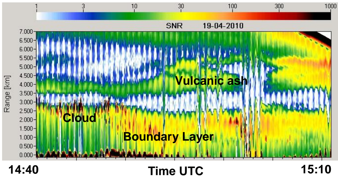
Figure 6: Quicklook from 2- \mu m lidar measurements from Falcon flight on April 19, 2010 showing Signal-to-Noise Ratio during 30 minutes south of Leipzig and around Leipzig from 14:40-15:10 UTC (16:40-17:10 LT); red/black colors show high SNR from clouds (around 3 km) and ground (0 km); blue-green colors show layers with aerosol; white/blue colors indicate noise (no valid data); the 2 layers of higher aerosol level (left side of Figure) at 4 and 5.5 km merge to 1 layer of almost 2 km thickness (right side of Figure).
