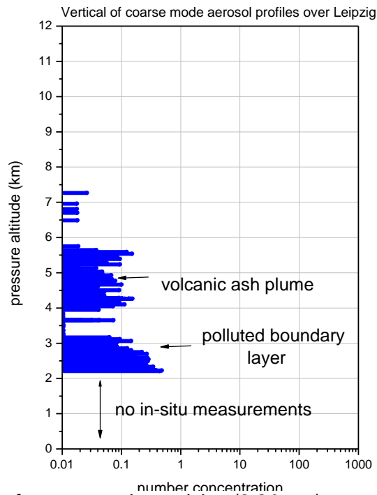
Figure 11: Vertical profile of coarse mode particles (3-20 \mu\text{m} ) measured over Leipzig.
