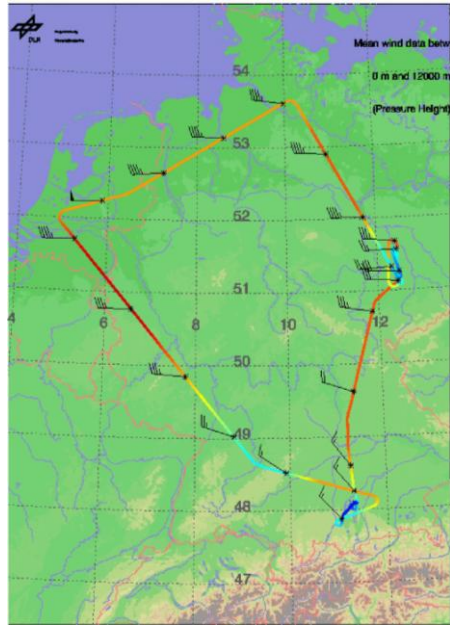
Figure 1: Flight route of the DLR Falcon on 19 April 2010
