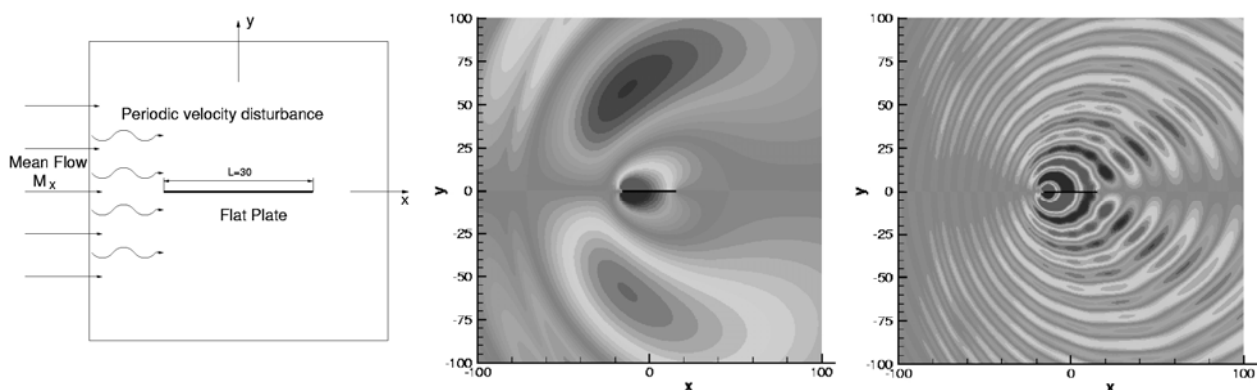
Sound generation at a flat plate due to incident gusts of different wave-lengths 16.02.10, Jan Delfs, R. Ewert
