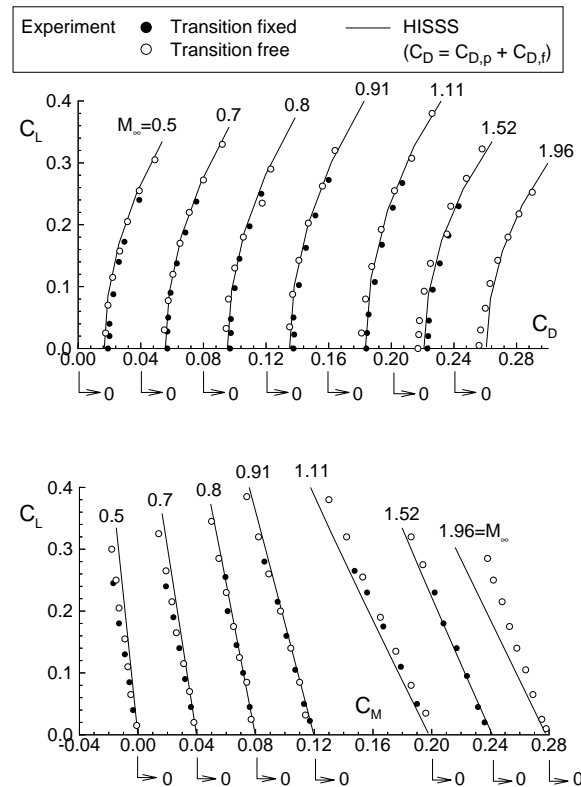
Fig. 8 HISS validation for slender supersonic configurations.
