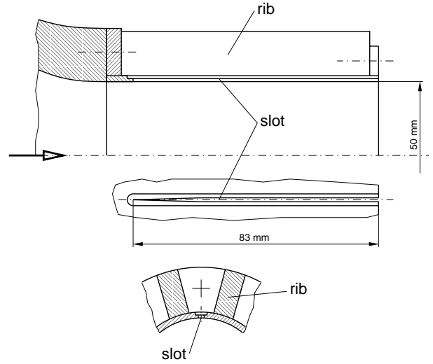
Figure 5: Sketch of the slotted nozzle
