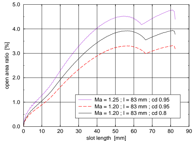
Figure 6: Open area ratio of slotted nozzle (total slot width to nozzle perimeter) for different design Mach numbers and discharge coefficients
