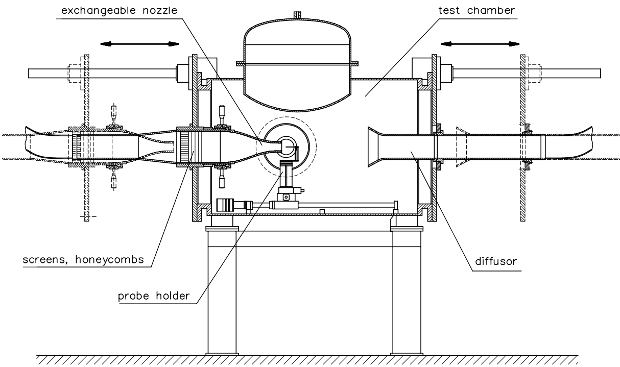
Figure 1: Test facility for probe calibration (SEG)
