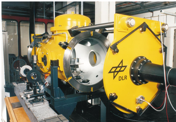
Figure 2: Photo of the open wind tunnel with a probe installed for calibration
