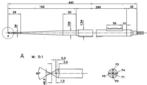
Figure 16: Sketch of the pyramid probe
