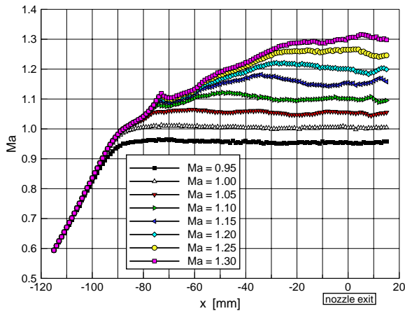
Figure 13: Mach numbers at the center line of the transonic nozzle
