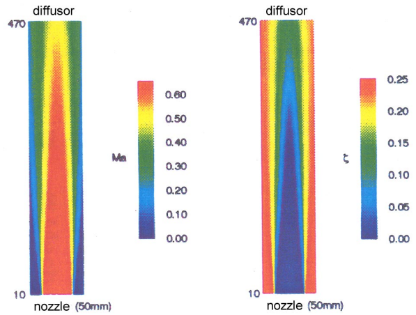
Figure 11: Local Mach number (left) and loss coefficient (right) of the free jet
