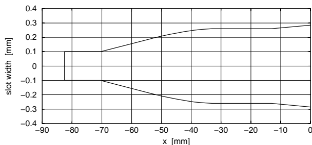
Figure 7: Actually manufactured slot: slot width of one slot is displayed as a function of the x-coordinate ( x = 0 at the nozzle exit)
