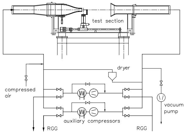
Figure 3: Circuit of SEG (schematic)
