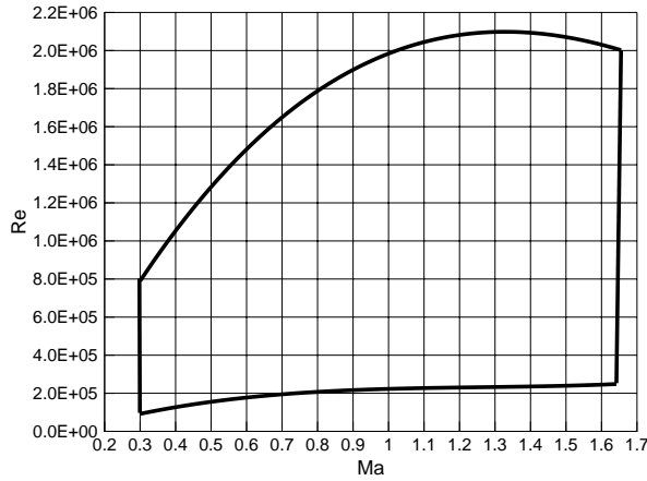
Figure 9: Range of Mach numbers and Reynolds numbers available for probe calibration up to now
