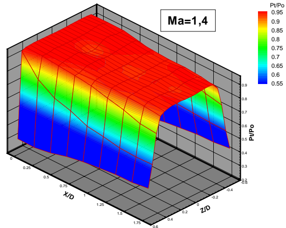
Figure 14: Total pressure downstream of the supersonic nozzle ( Ma = 1.4 )
