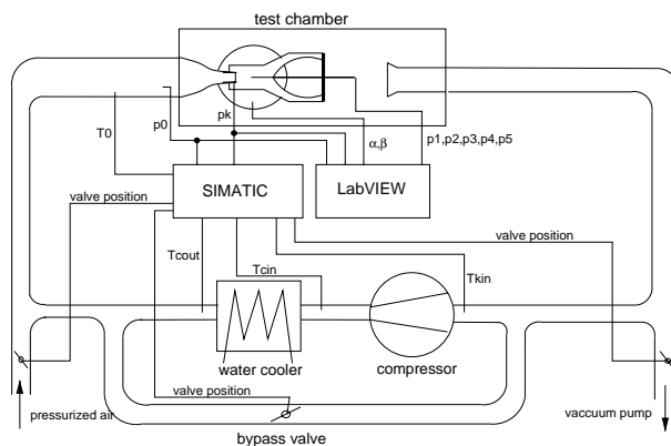
Figure 8: Flow control and data acquisition at SEG (schematic)
