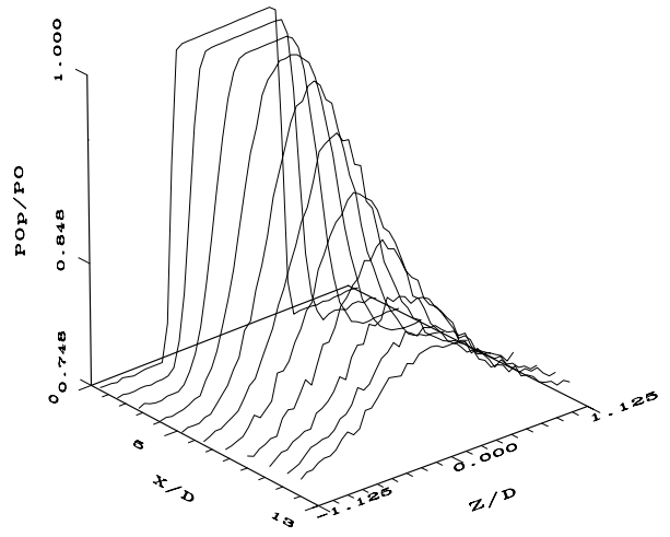
Figure 10: Total pressure of the free jet
