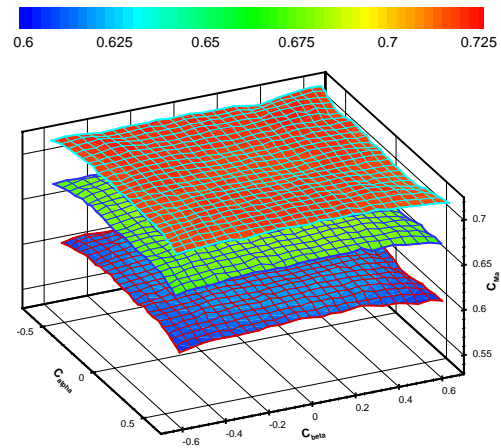
Figure 17: Measured coefficients at Ma = 0.7, 0.8, 0.9
