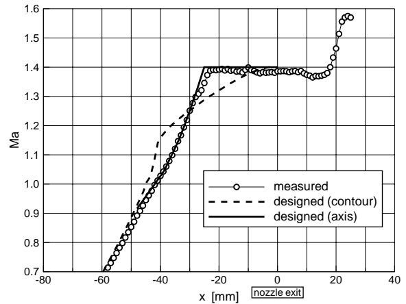
Figure 15: Mach numbers at the center line of the supersonic nozzle Ma = 1.4
