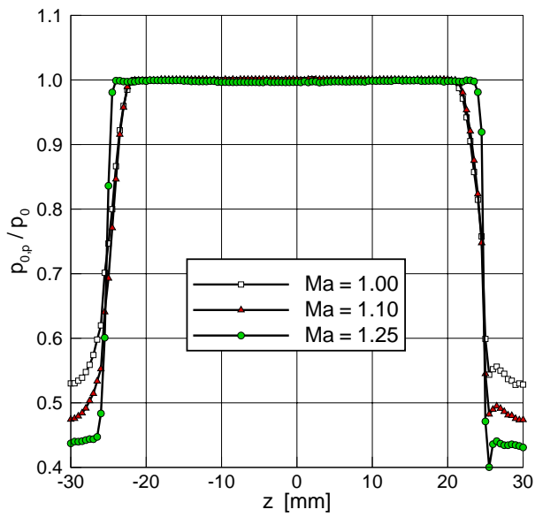
Figure 12: Total pressure downstream of the transonic nozzle ( x = 2mm )
