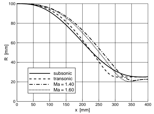
Figure 4: Contours of different nozzles
