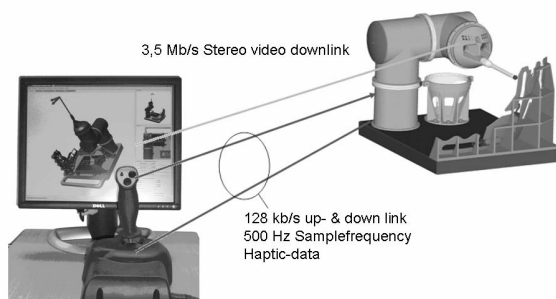
Fig. 3 Telepresence based upon DLR's high-fidelity force reflecting joystick and stereo visual feedback
