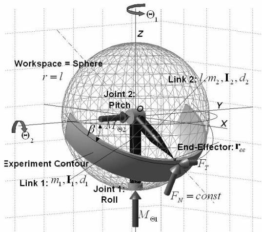
Fig. 16 ROKVISS manipulator: contact case, stylus moving on a given trajectory. This figure is part of an animation: the length of the arrows is varying according with time. The arrows indicate the torques of the two joints exerted during motion and the reaction force at the contact surface.
