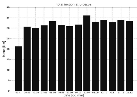
Fig. 13 Time evolution of total friction at a speed of 5deg/s. The first bar corresponds to the reference measurement on ground.
