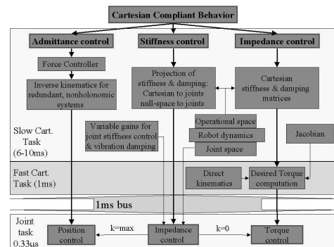
Fig. 10 Controller architecture
