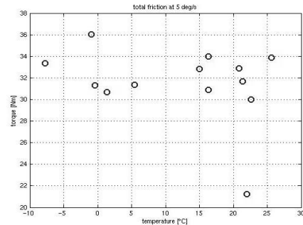
Fig. 14 Total friction at 5deg/s, plotted over the temperature. The isolated value corresponds to the reference measurement on ground.
