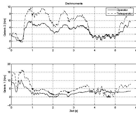
Fig. 8 Recorded torques contour following
