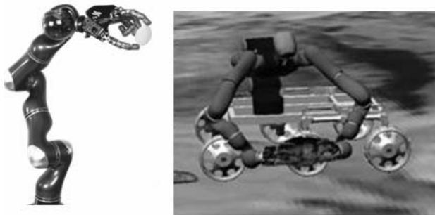
Fig. 19 DLR's operational light-weight arm/hand system (left) and a humanoid planetary rover concept based on DLR's light-weight arm/hand system (right)
