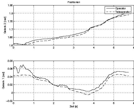
Fig. 7 Recorded positions during contour following
