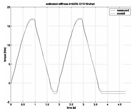
Fig. 15 Result of stiffness optimization.
