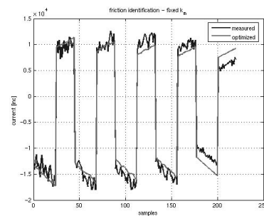
Fig. 11 Commanded current and current estimation after the identification of the friction parameters. The movements are performed with 30.0, 20.0, 10.0, 5.0, and 1.0deg/s.
