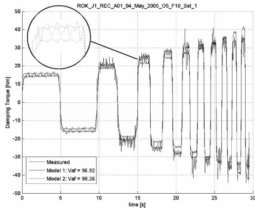
Fig. 12 Two different models for the friction torque are compared. Vaf (= variance accounted for) defines a statistical measure to judge to quality of the identification results and hence the underlying model: The ideal value vaf=100% means that we have total agreement between model and measurement.
