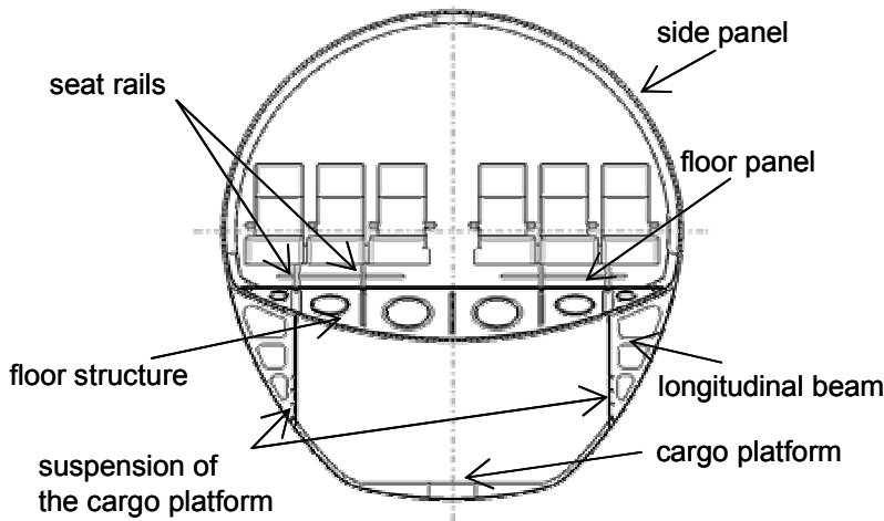
Figure 1: Cross-section of the CFRP fuselage built according to the Gondola concept
