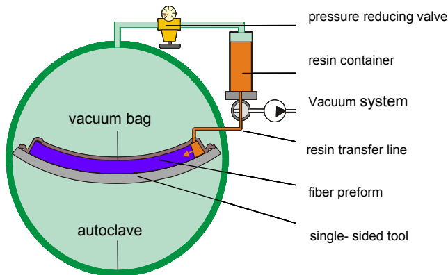
Figure 4: Single-line injection principle (SLI)
