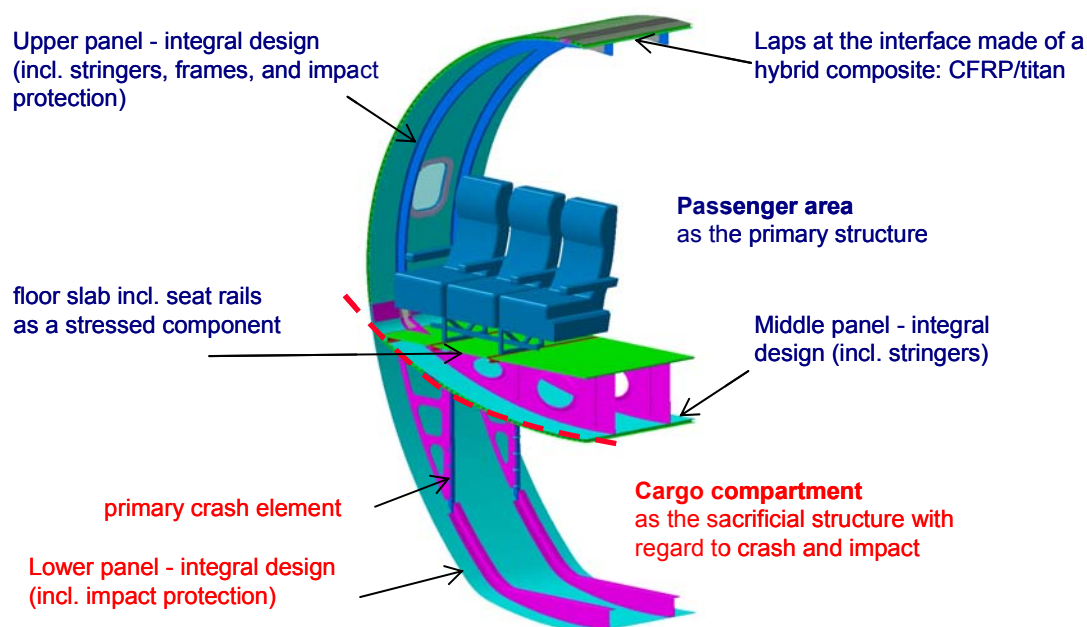
Figure 3: CFRP fuselage demonstrator
