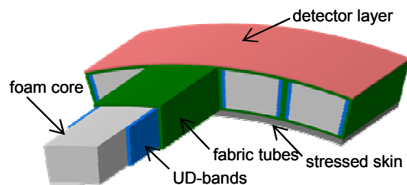
Figure 7: Set up of the shells
