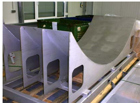
Figure 5: Tooling for the fuselage shells
