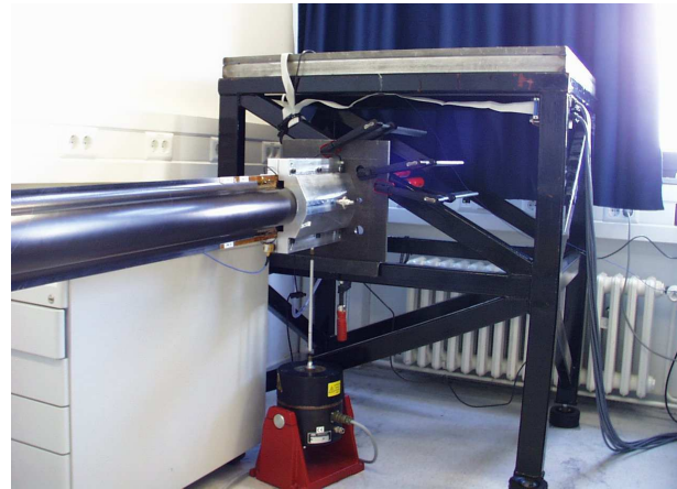
Fig. 10: Test stand with the adaptive boom supported in cantilever form (length approx. 2 m).
