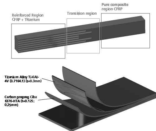
Figure 2. Hybrid Material Configuration
