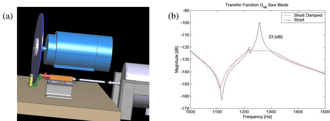
Fig. 14: (a) Test set-up of cutting saw, (b) Simulated vibration reduction
