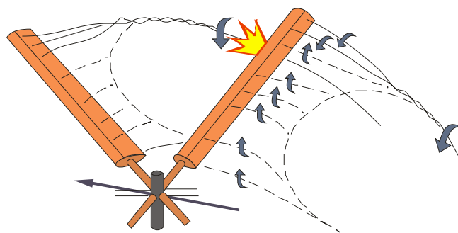
Fig. 7: Blade Vortex Interaction (BVI)
