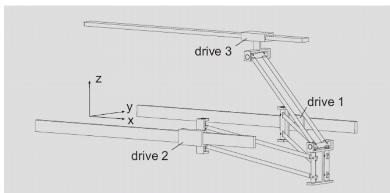
Fig. 13: Triglode parallel robot
