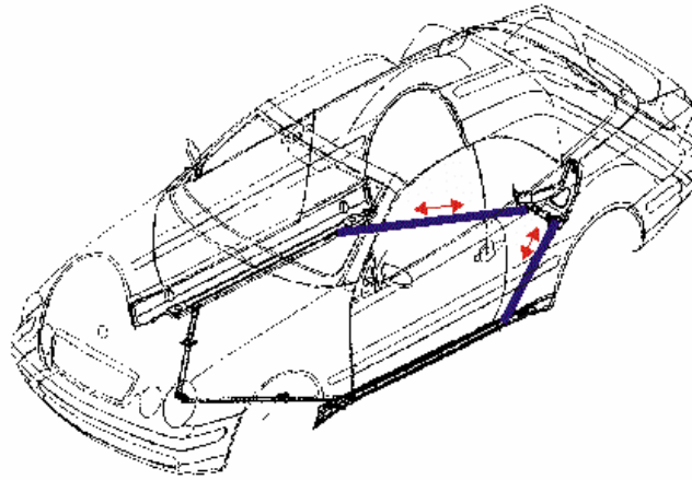
Fig. 6: Active Rods embedded in the frame of the body
