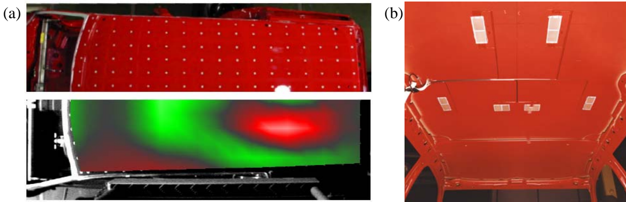
Fig. 5: (a) Experimental modal analysis, (b) Attached piezoceramic patches
