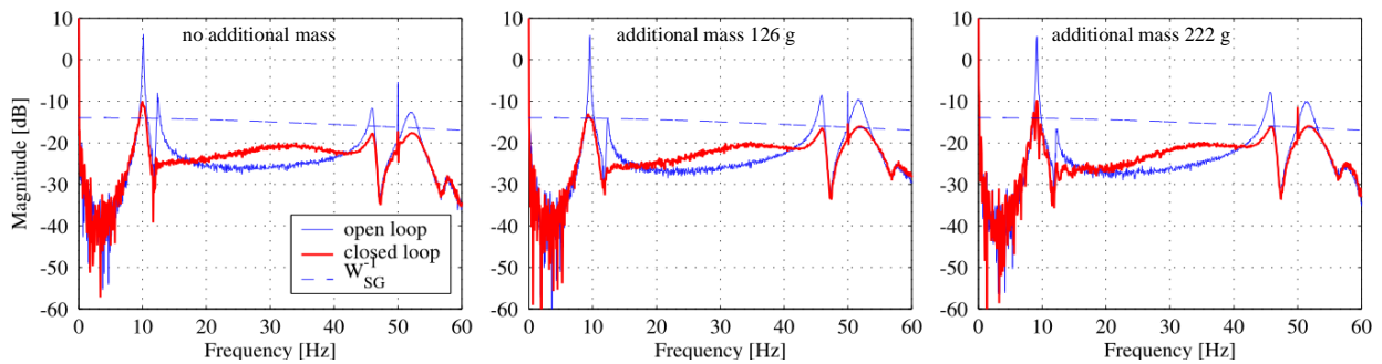
Fig. 12: Open- and closed-loop FRF
