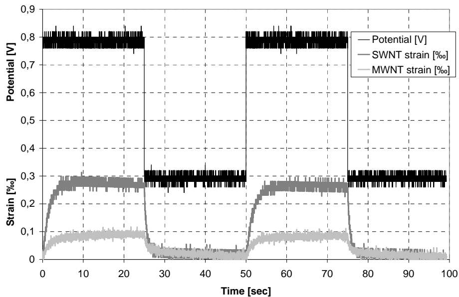
Fig. 4: System input (voltage step) and strain response for Single- and Multiwalled Nanotubes (SWNT/MWNT)
