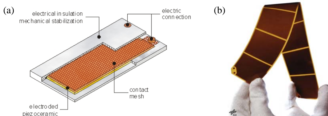
Fig. 2: (a) Principle design of encapsulated patch, (b) Special shaped actuator
