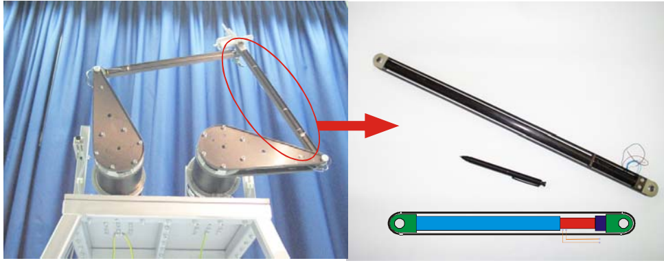
Fig. 11: The Five-Bar parallel robot (left), active rod (right)
