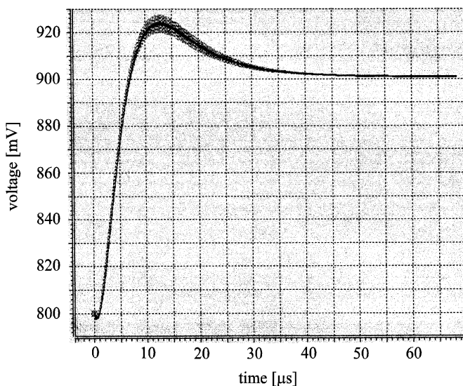
Fig. 8. Input step response
