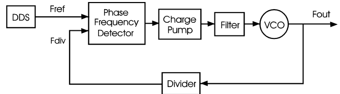
Fig. 1. Block diagram of the frequency synthesizer.
