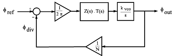
Fig. 2. System level model of the PLL
