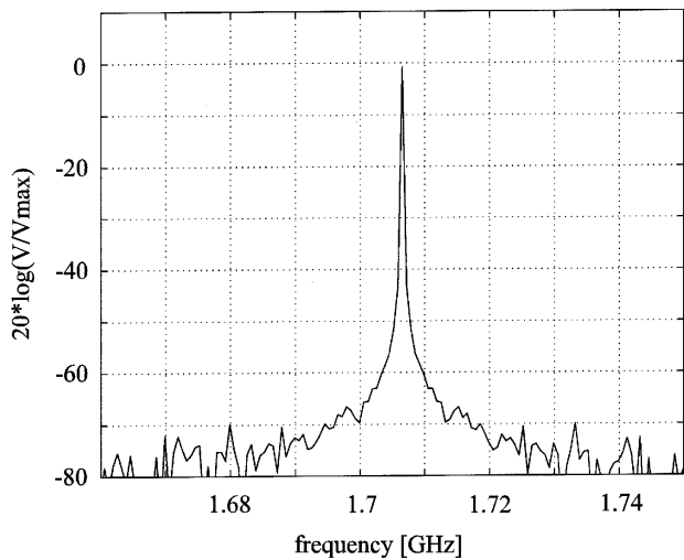
Fig. 9. Simulated output spectrum of the frequency synthesizer
