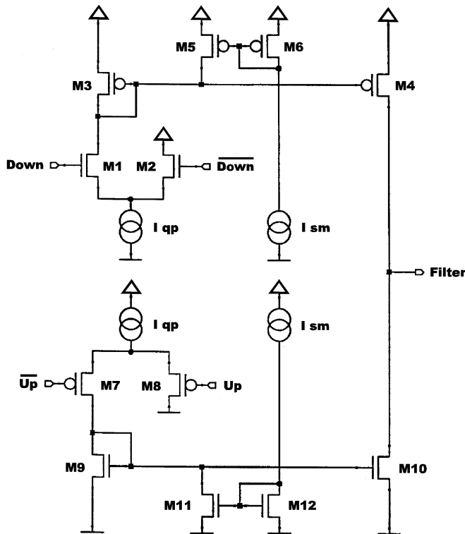
Fig. 4. Simplified schematic of the charge pump circuit.
