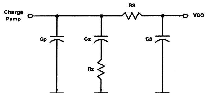
Fig. 5. Loop filter
