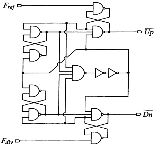
Fig. 3. Phase-frequency detector without dead zone.
