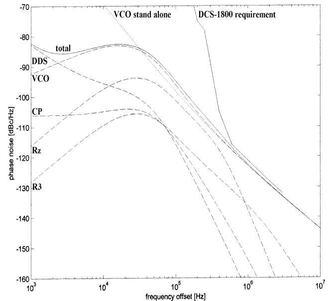
Fig.7. Output phase noise due to various sources
