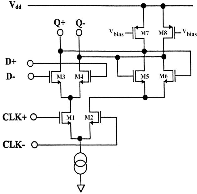
Fig. 6. D-Latch in prescaler circuit
