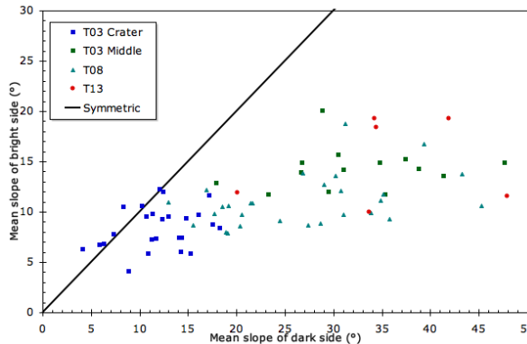
Figure 2. Slopes on the bright and dark sides of 76 Titan mountains, as estimated by radarclinometry. The average slope of a relatively straight and representative segment of several pixels is used, to avoid the bias of extreme 1-pixel slopes by noise. Note the increase of asymmetry with slope.
