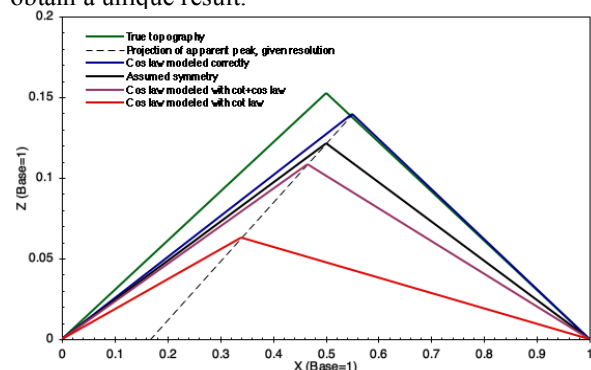
Figure 3. Idealized model of a symmetric mountain, seen in cross-section in a plane of constant radar azimuth. Radar illumination is from the left. The figure shows the true profile (green) and profiles recovered under the assumption of symmetry and by radarclinometry with various scattering laws. In this case ( i = 20^\circ , \theta = 16^\circ , resolution = 1/6 of mountain width) the bright face is unresolved but is not folded over. These profiles illustrate one case drawn from the parametric plots in Figs. 4-5.
