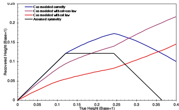
Figure 4. Estimated height of mountains imaged at i = 20^\circ as a function of true height, as obtained by assumed symmetry and by radarclinometry with correct and incorrect scattering law assumptions.
