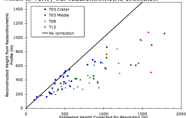
Figure 6. Corrected and uncorrected heights of Titan mountains. The correction factor is based on the assumption that dark slopes have been estimated correctly, as is the case for our simple mountain models.
