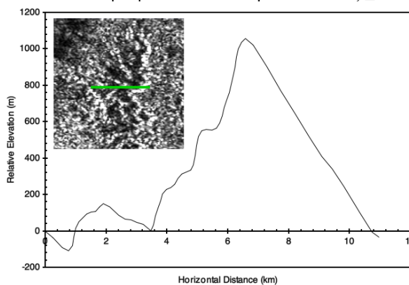
Figure 1. Example of a Titan mountain in Cassini RADAR T8 image (illumination from right) and radarclinometric profile at location in green. Note vertical exaggeration.
