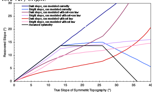
Figure 5. Estimated bright and dark side slopes of mountains imaged at i = 20^\circ as a function of true slope, for same modeling assumptions as Fig. 4. Note that the dark side slope is recovered accurately when the correct scattering law is used (dark blue line).
