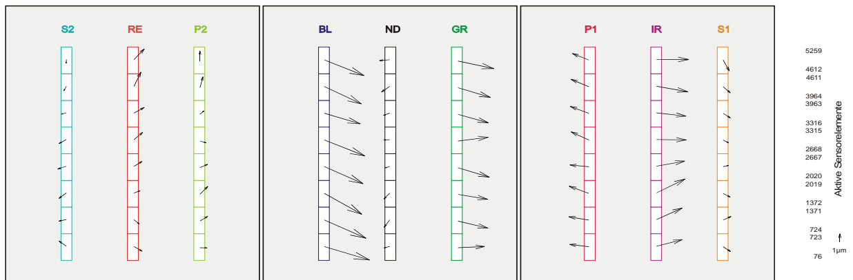
Figure 3: Systematic residuals at the image coordinates (orbit 2063) before adjustment of interior orientation. Each of the 9 lines is divided in 8 parts. For these parts the root mean square error is showed.
