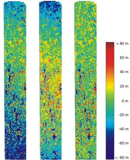
Figure 2: Z-differences between HRSC Object points and MOLA DTM of orbit 2063. Before bundle adjustment (left), after bundle adjustment using with calibrated interior orientation (middle) and after bundle adjustment using the new interior orientation (right).
