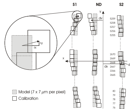
Figure 1: Relationship of dx , dy , rx , and ry .
