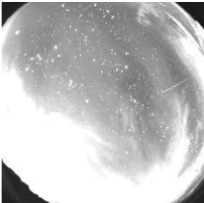
A single meteor detected in 5 consecutive images (4-5 seconds)
