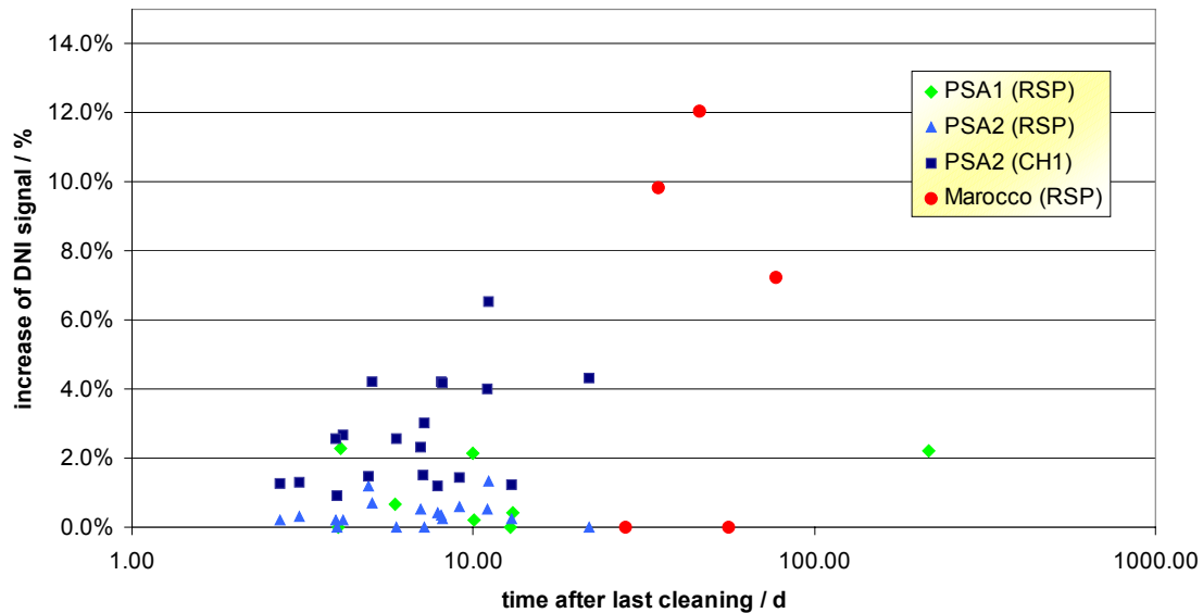
Figure 7: Soiling of sensors: increase of the DNI signal by cleaning different sensors at different sites in dependence of the time period after the last cleaning.
