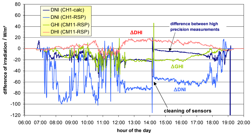
Figure 6: Difference of the measured and calculated DNI signal from the high precision instruments as well as the deviations of the RSP signals as subtracted from the measurements of the precision instruments. Measurements from the 19th of September 2002 taken at the PSA. At 14:10 the sensors have been cleaned.
