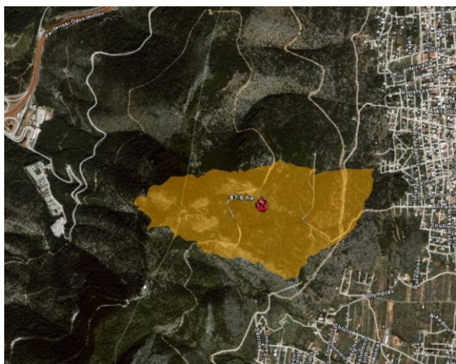
Figure 3: Ymittos forest – Greece : Burn scar map (fire contour).
