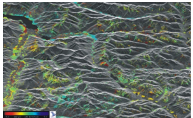
Figure 2: Example of (PSInSAR) radar data colours point out ground displacements
