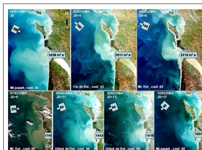
Figure 2: Gironde plume as a function of water discharge (© GEOtransfert)
