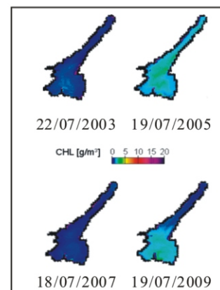
Figure 2: Maps of Chlorophyll in Garda lakes Obtained by MERIS images
