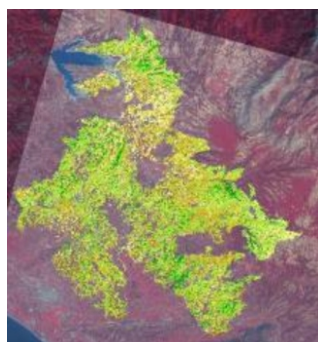
Figure 1: Analysis of the land cover classes distribution inside the burnt area (including statistics over burnt areas per type of land cover class).
