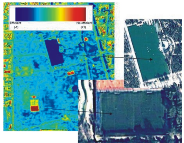
Figure 2: Temperature map of Retiro Park in Madrid City
