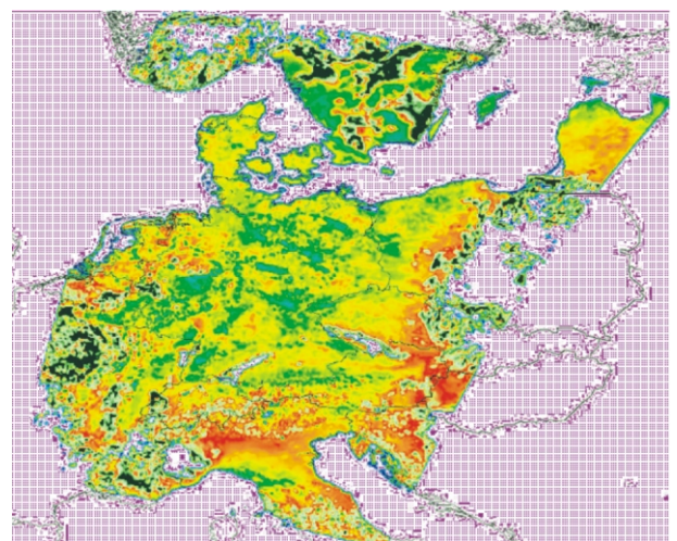
Fig. 1: PM 10 concentration over Europe (Image under creative-commons license: by-nc-nd)
