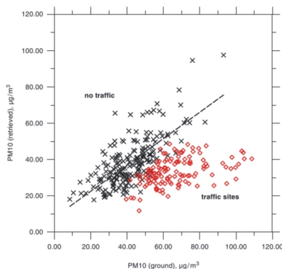
Figure 2: Comparison of cloud-screened retrievals of PM10 from MERIS scene of October 13, 2005 and ground-based measurements of PM10 concentrations for the MERIS over flight time, provided by the German Federal Environmental Agency (Umweltbundesamt). For the traffic sites no correlation is found between satellite-derived and ground data.
