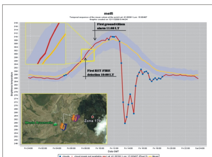
Figure 2: Example of RST timely detection during the 2009 real-time validation campaign: the Melfi (Potenza) event. In the plot, the daily MSG-SEVIRI MIR signal compared to its expected value. In the inset, the two thermal anomalies detected at 08:00GMT, one hour before the first alarm.
