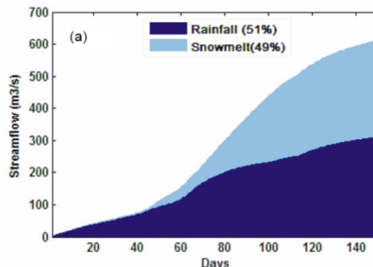
Figure 3. Snow melt and stream flow modelling: Respective contributions of rainfall and snow to the flow of the Ourika River, Morocco
