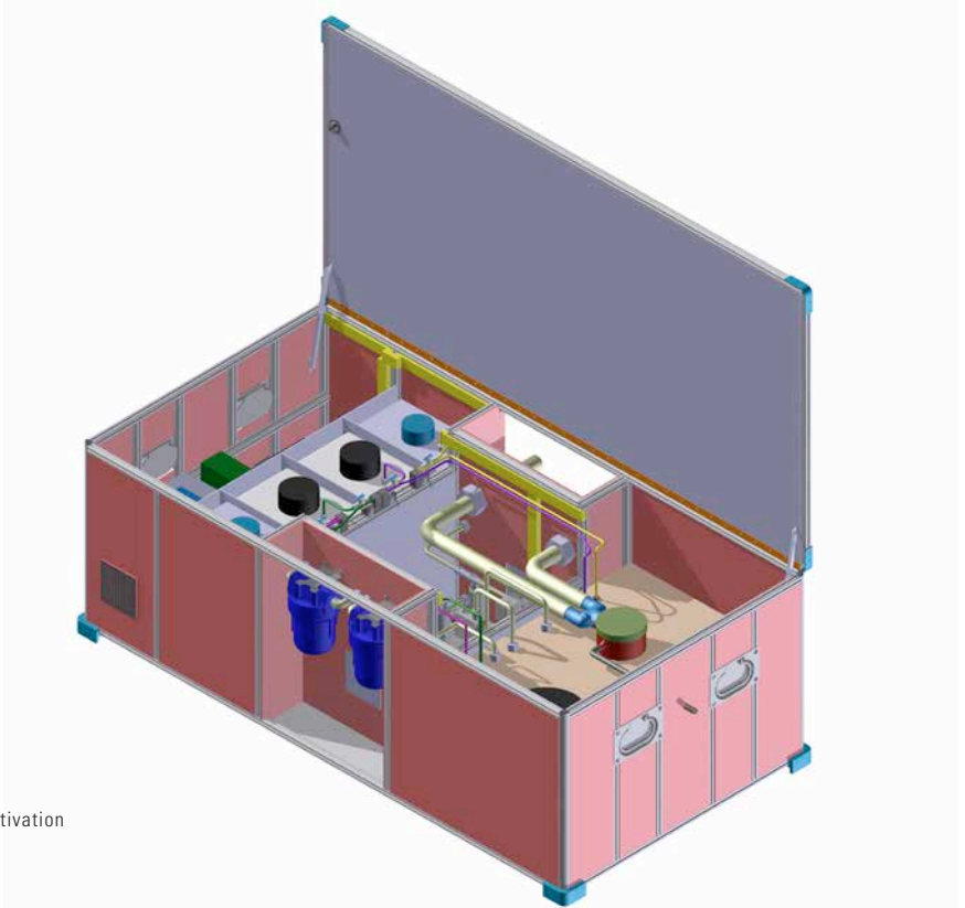
Render of the MEPA Controlled Environment Agriculture support unit
