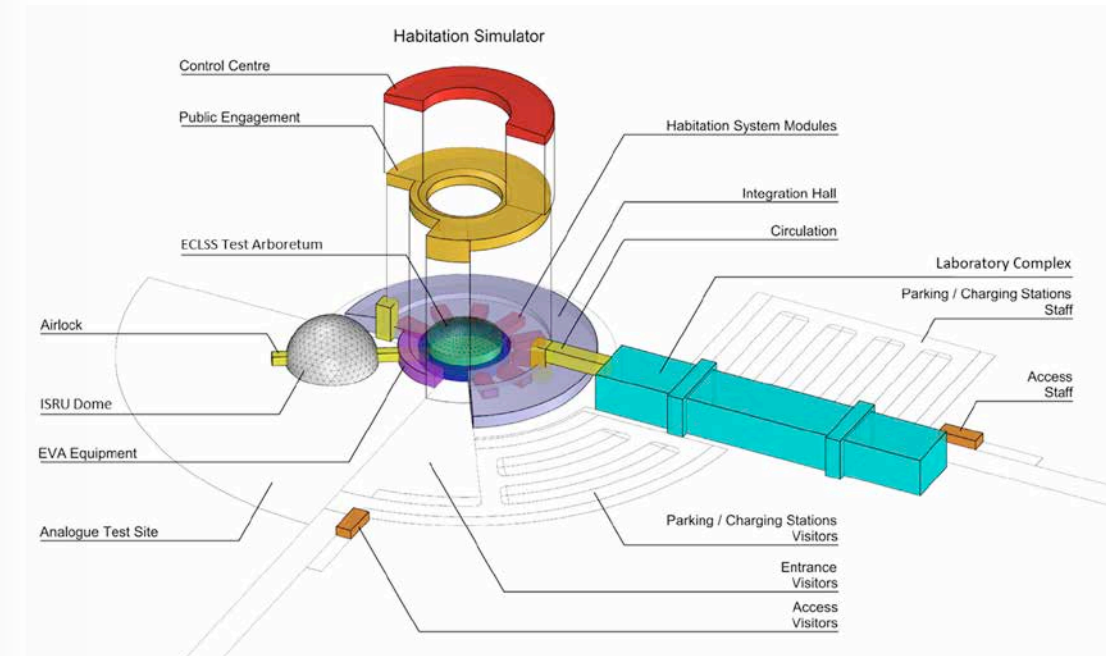
Overview of the Incubator for Habitat- and Sustainability Technologies (IHST) design (credits:Rene Wacławicek, Liquifer Systems Group)
