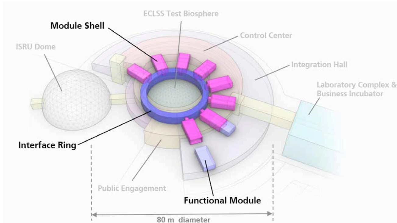
Functional layout of the habitat simulator inside the IHST (credits:Rene Wacławicek, Liquifer Systems Group)
