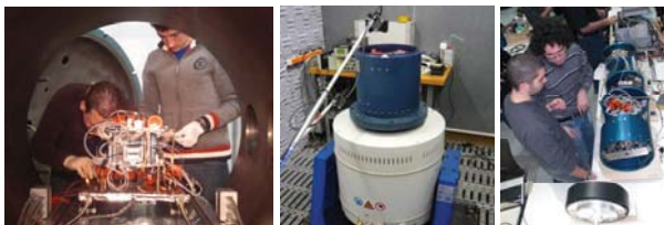
Figure 9. Vacuum chamber (left), shaker (middle), service system simulator (right).
