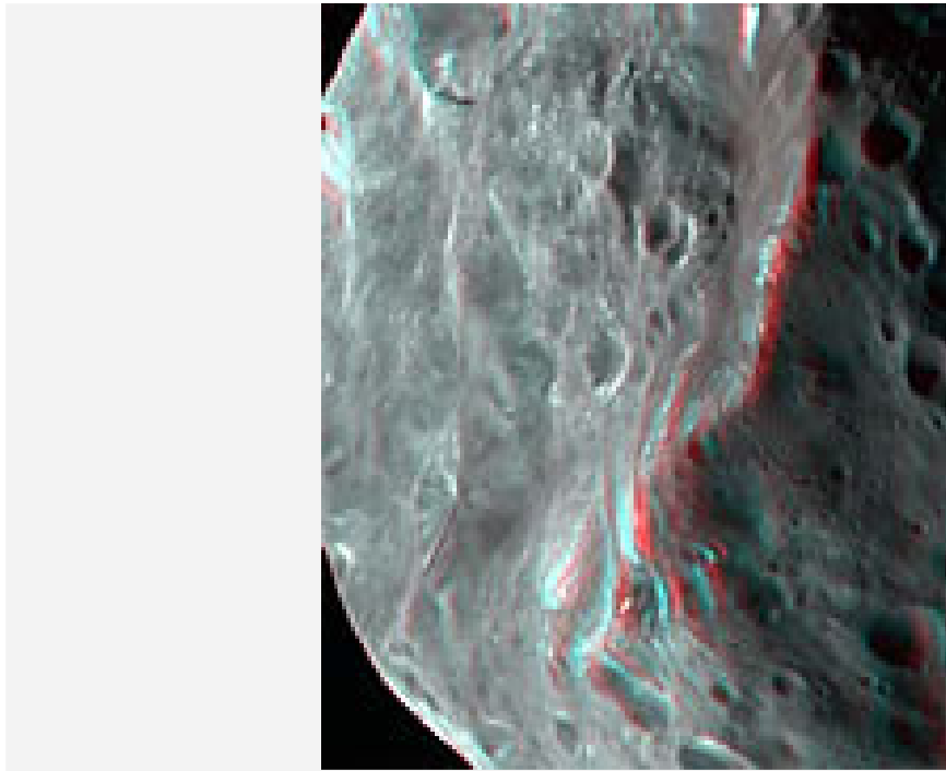
Phoebe's largest crater in 3-D
