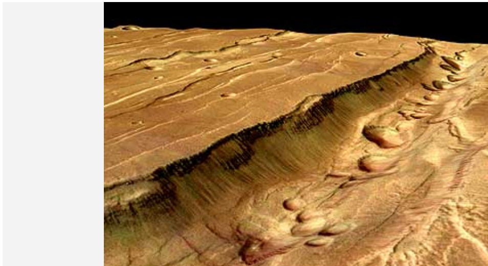
Perspective view of Phlegethon Catena
