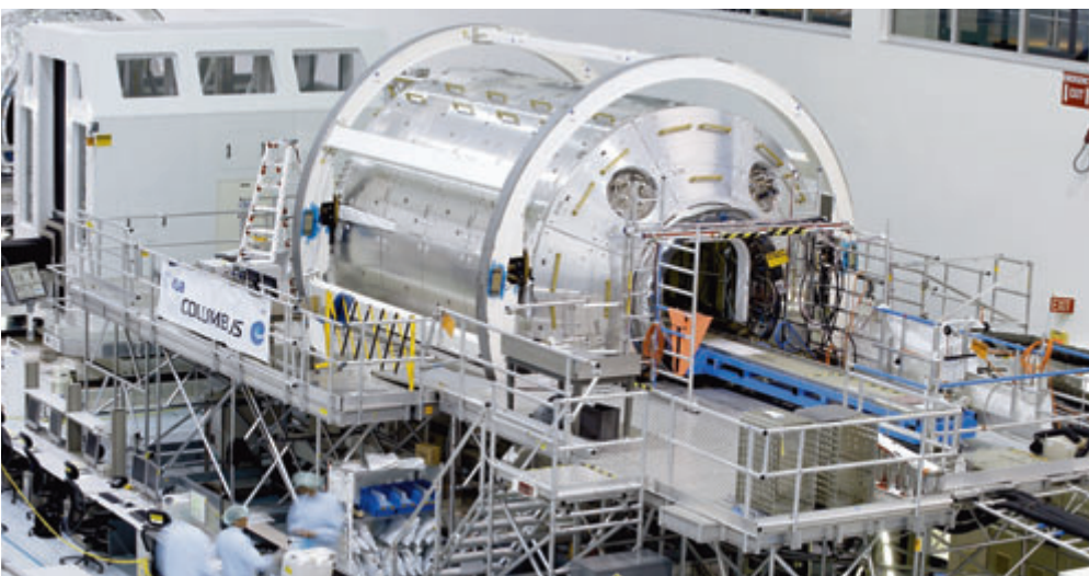
COLUMBUS in der ISS-Vorbereitungshalle COLUMBUS at the Space Station Processing Facility
