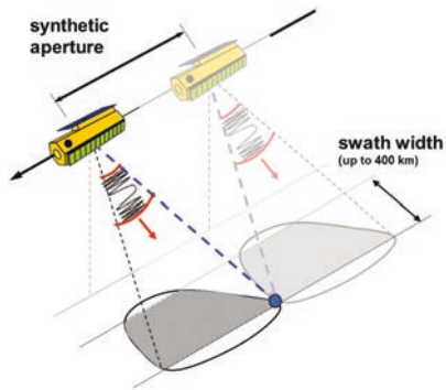
Synthetic aperture radar (SAR). The formation of a synthetic aperture several kilometers long enables a high-resolution independent of range to be achieved.
