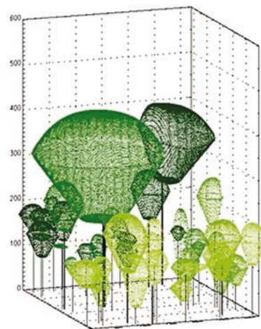
3D representation of a primary tropical forest having a natural structure using the example of a dipterocarpaceen forest on Borneo, Indonesia. Tandem-L will measure the vertical forest structure on a global scale.
