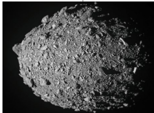
Brace for impact! A mosaic of the last images from the DART probe before it hit Dimorphos. The asteroid's 'rubble-pile' morphology is clearly visible.
