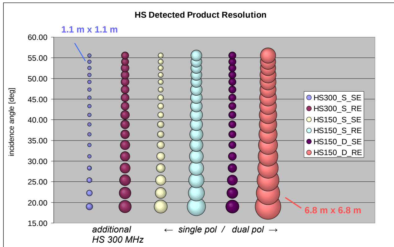
Fig. 3-5: The relative resolutions of detected product variants for the HS modes as they depend on the incidence angle.
