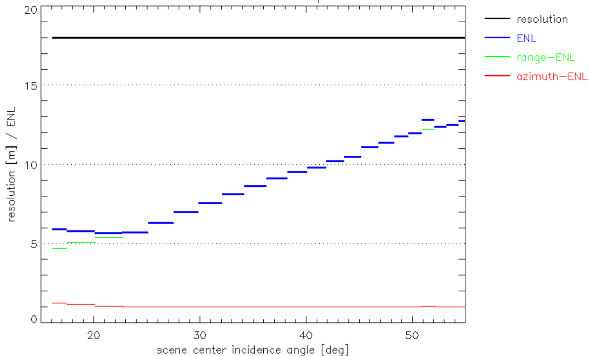
SC S 150MHz RE Products : Resolution & Equivalent Number of Looks
