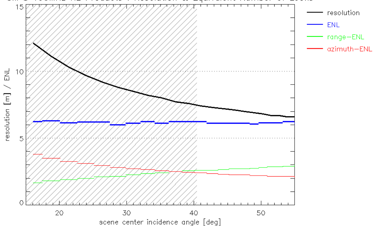
Fig. 4: Stripmap single polarization RE product variant for 100 MHz range bandwidth.
