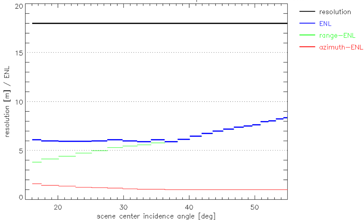
SC S 100MHz RE Products : Resolution & Equivalent Number of Looks
