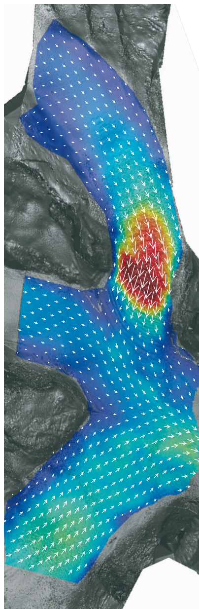
Measurement of glacial velocities using the Aletsch glacier (Switzerland) as an example. The information was derived from airborne L-band data.
