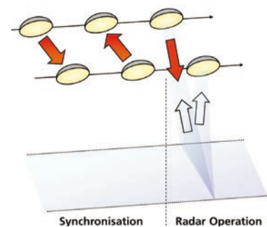
To synchronise the radar systems, short pulses are exchanged between the satellites. This permits a synchronisation to a picosecond.
