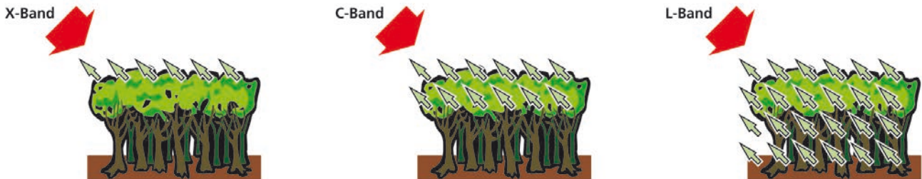
Comparison of the penetration depth in vegetation for X, C and L-band with 3 cm, 5 cm and 24 cm wavelength. While radar waves in X-band are only reflected from the upper canopy, L-band penetrates down to the ground. Only L-band radar systems can receive signals from all parts of the vegetation.
