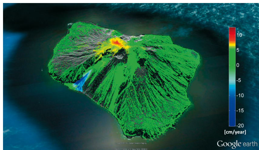
Deformation of the volcano Stromboli in Italy in cm/year. The use of both point targets and distributed targets yields a particularly high information density.
