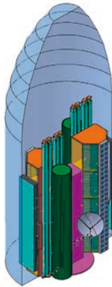
Two Tandem-L satellites in the fairing of a Falcon 9
