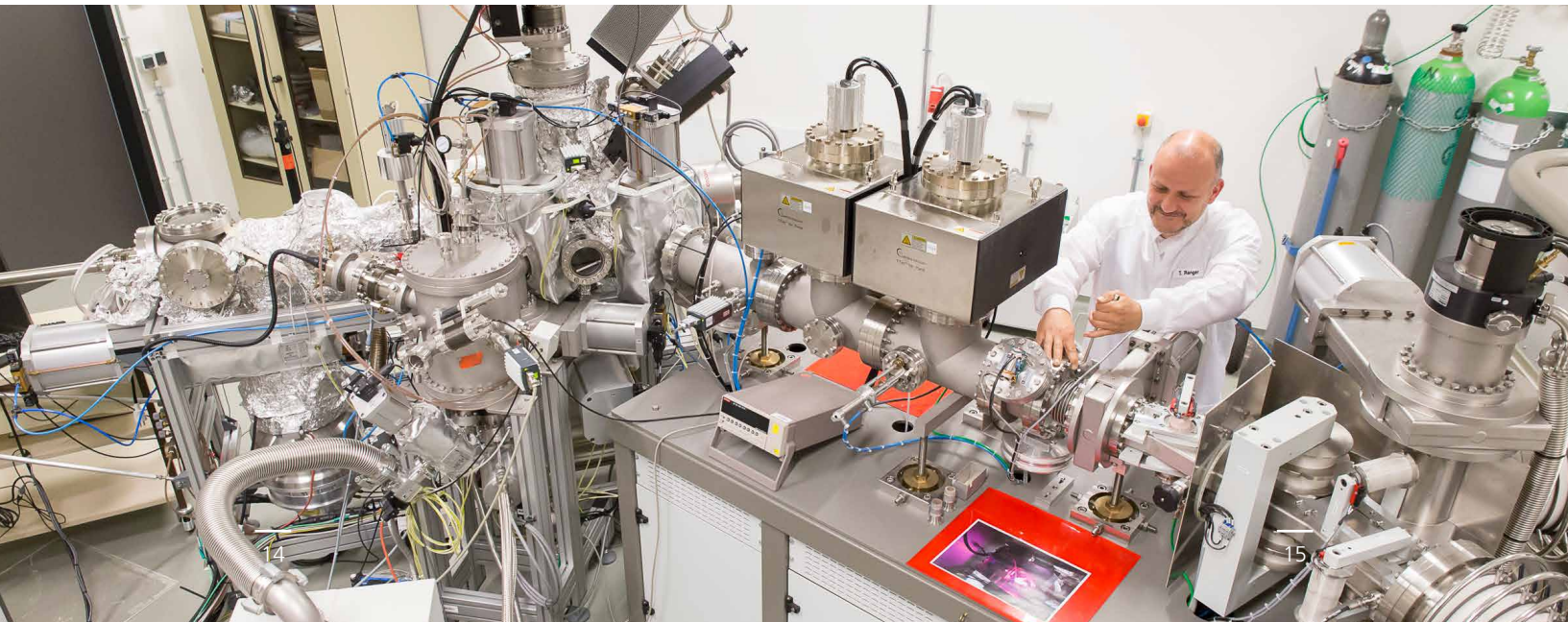
The Complex Irradiation Facility (CIF)
