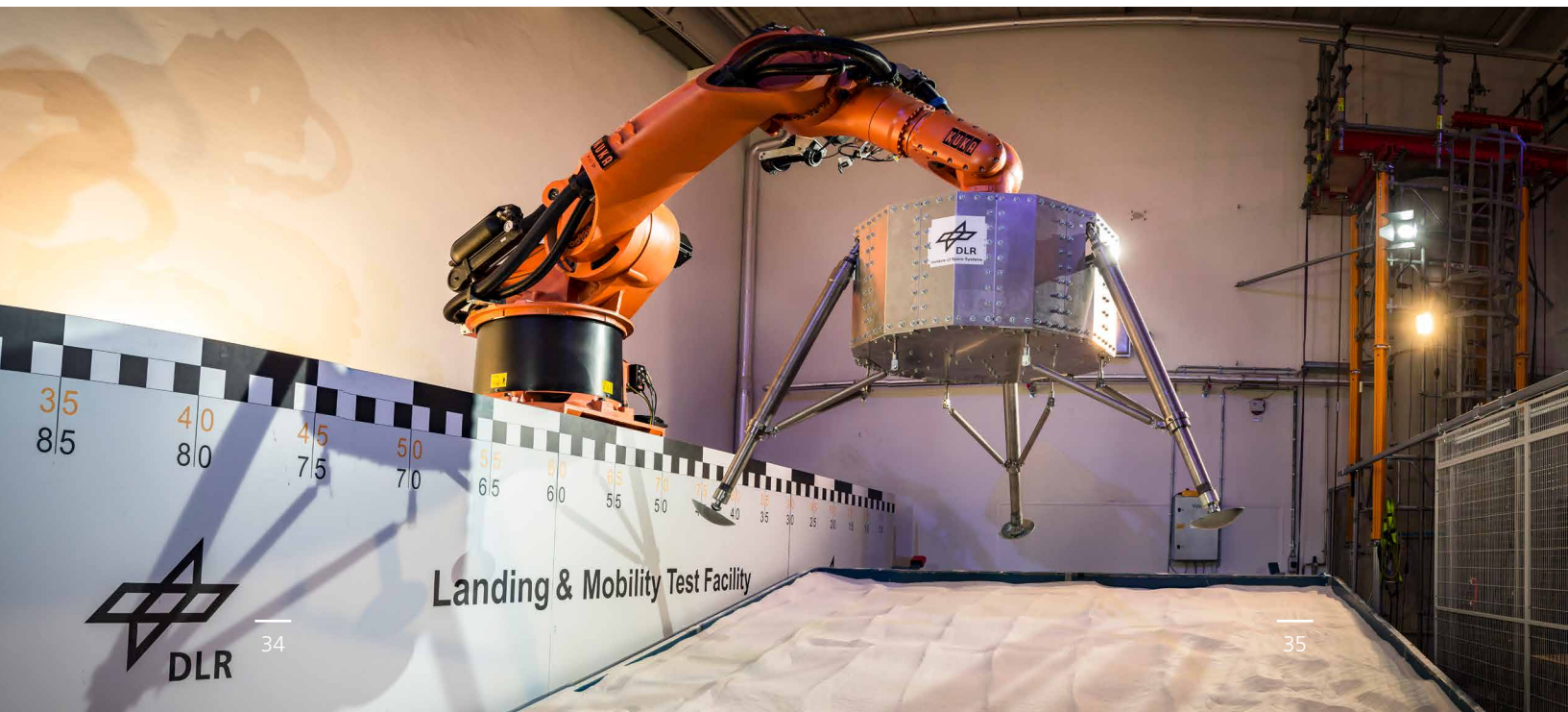
LAMA with Lander Engineering Model
