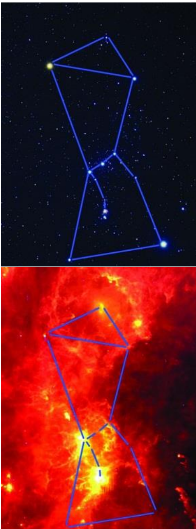
Fig. 8: The star constellation Orion as seen in the visible spectrum (a) and the infrared spectrum (b). Gas and dust nebulae in the centre are regions in which new stars are born. (Picture: Akito Fujii und IRAS)
