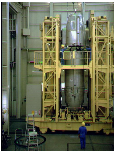
Drop capsule in Japanese Microgravity Center Kamisunagawa
