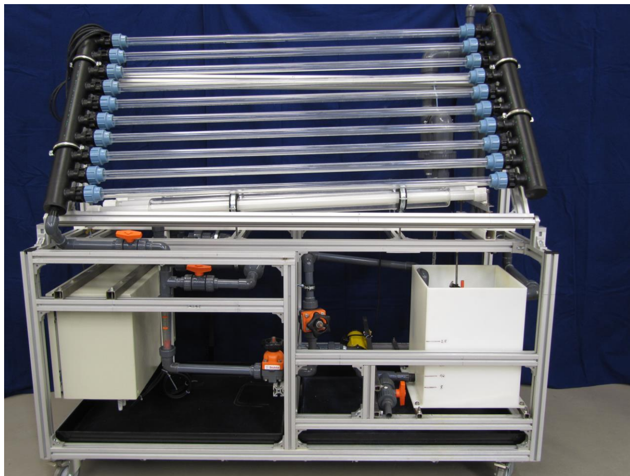
The apparatus for solar water purification in the DLR_School_Lab Cologne combines two reactors: The ten sloping tubes can be used to carry out the experiment using sunlight. Underneath, three almost horizontal tubes carry the chemicals when artificial UV light is used. The bottom of the apparatus carries (from left to right) a switchboard, valves, the pump (yellow) and tank for the reactants.
