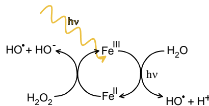
Photo-Fenton-reaction
