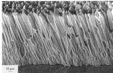
Ceramic coating on a compressor blade
